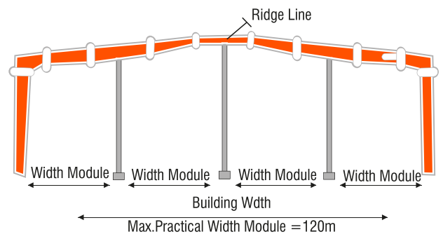
TAPERED COLUMN MULTI SPAN "3" (TCMS-3)
