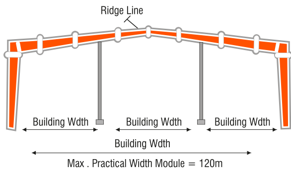
TAPERED COLUMN MULTI SPAN "2" (TCMS-2)
