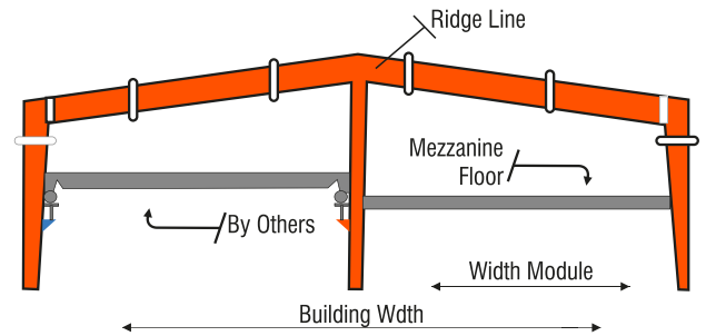
Crane Bracket & | Crane Beam / Mezzanine Floor Provision
