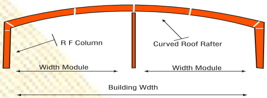
Arched Multi Span
