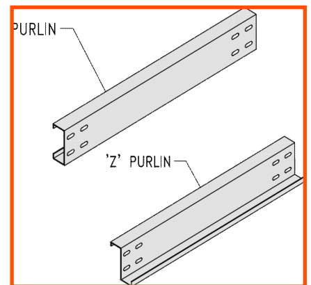
Ramji Purlins
